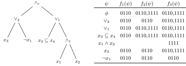
■ Figure 3 The table (Right) indicates subteams for each \psi \in \text{SF}(\phi) (Left). The teams f_1(\psi) and f_3(\psi) are propagated top-down whereas f_2(\psi) is propagated bottom-up. For brevity we omit subformulas x_1 and x_2 of x_1 \wedge x_2 .
