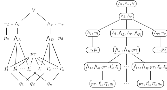
■ Figure 6 The Gaifman graph (Left) and a tree decomposition (Right) for \phi_{\mathcal{F}} . Note that we abbreviated subformulas in the inner vertices of the Gaifman graph for presentation reasons. Also, edges between p_{\top} and variables q_i are omitted for better presentation, but those are covered in the decomposition on the right.
