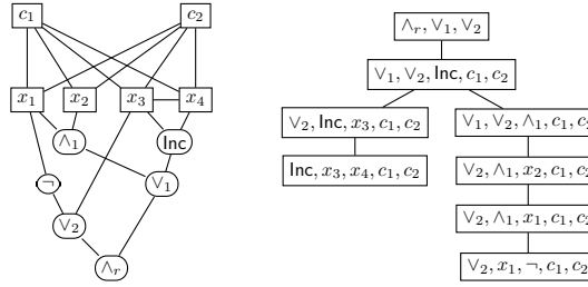
■ Figure 2 The Gaifman graph for \langle T, \Phi \rangle (Example 4) with a possible tree decomposition.
