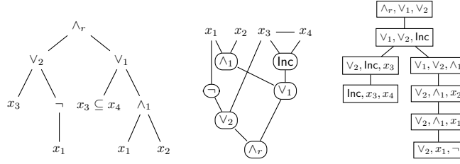
■ Figure 1 An example syntax tree (left) with the corresponding Gaifman graph (middle) and a tree decomposition (right) for (x_3 \vee \neg x_1) \wedge (x_3 \subseteq x_4 \vee (x_1 \wedge x_2)) . We abbreviated subformulas in the inner vertices of the Gaifman graph for better presentation.
